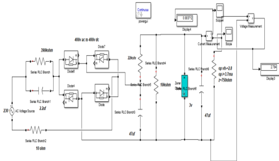
Figure.2 Simulation Circuit of Proposed topology in MATLAB.
